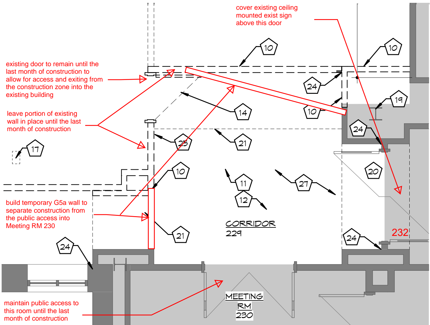
1D101 Partial Demolition Plan, not to scale
